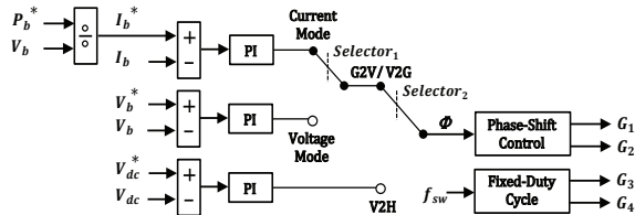
Figure 4. Control block diagram of the DAHB DC-DC converter based on PI compensators and the SPS technique
